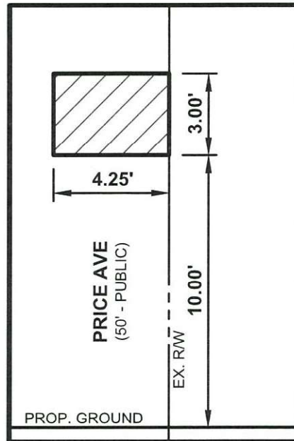
VERTICAL DETAIL (SCALE: 1" = 5')
