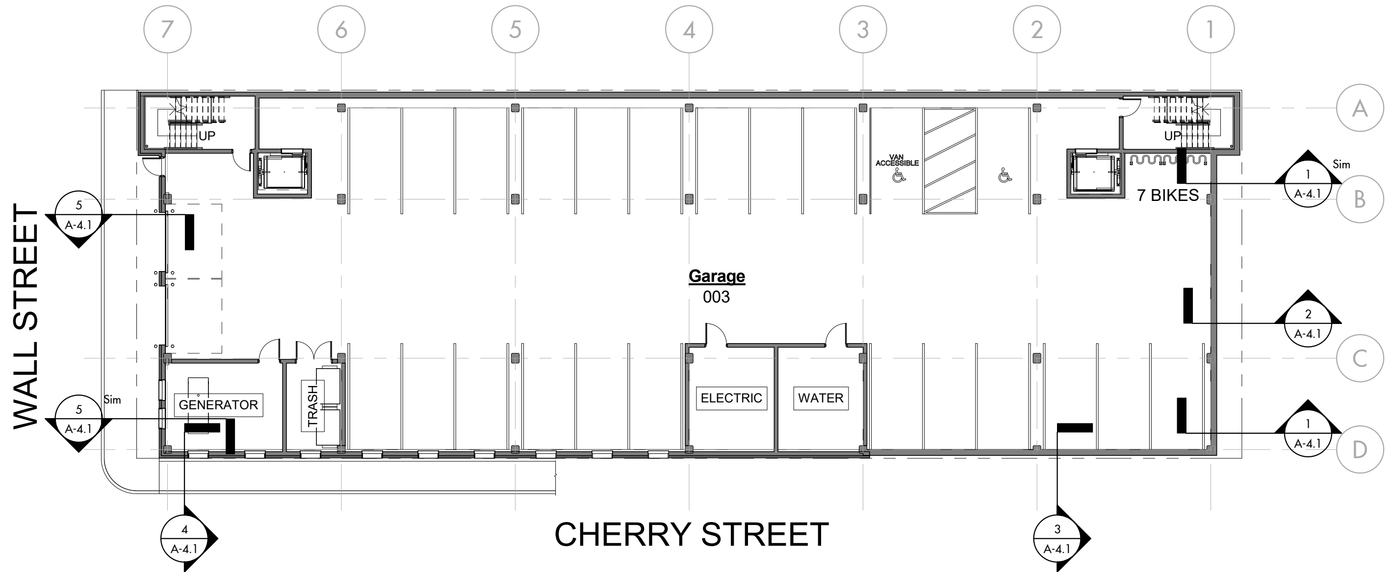
Floor 0 Plan 1/16" = 1'-0"
