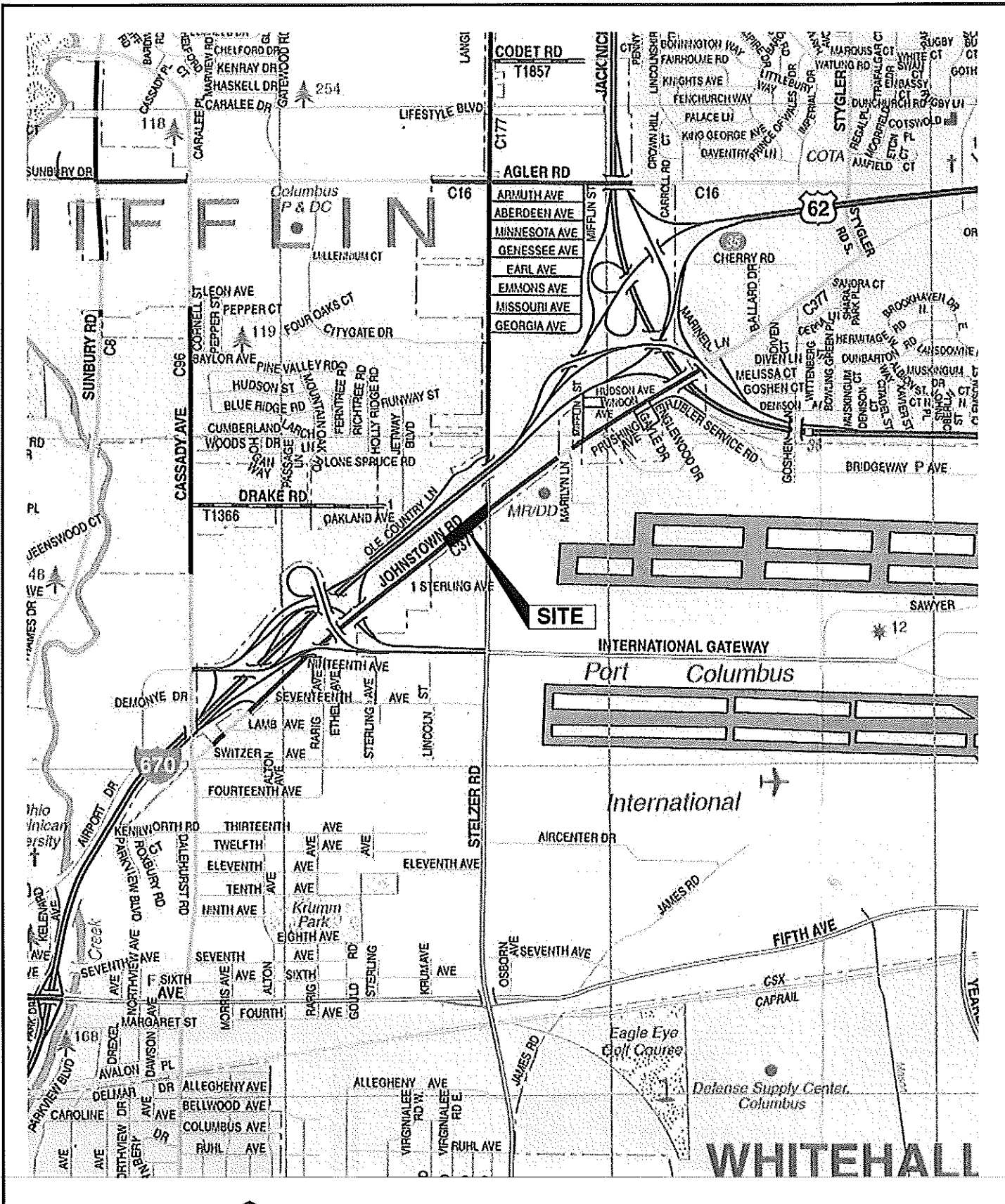
SITE MAP Johnstown Road Water Line Replacement Project
