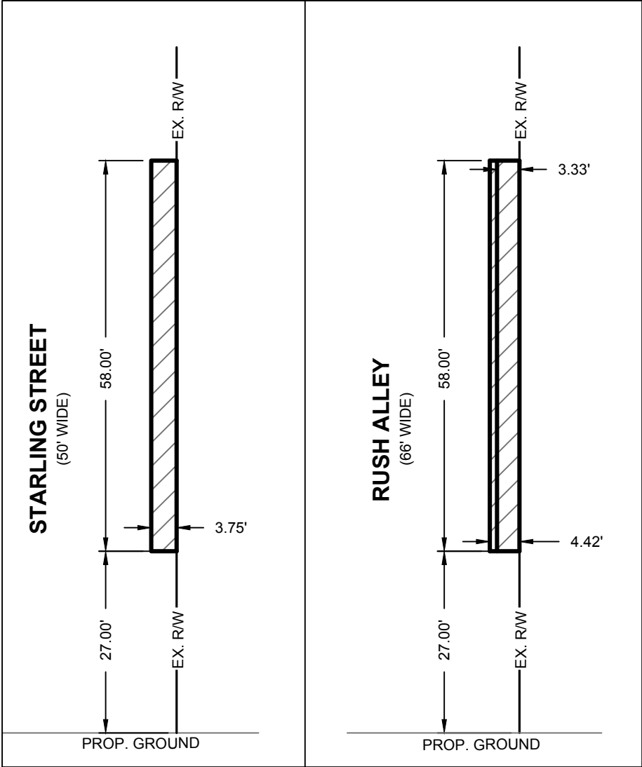
VERTICAL DETAIL (SCALE: 1" = 20')
