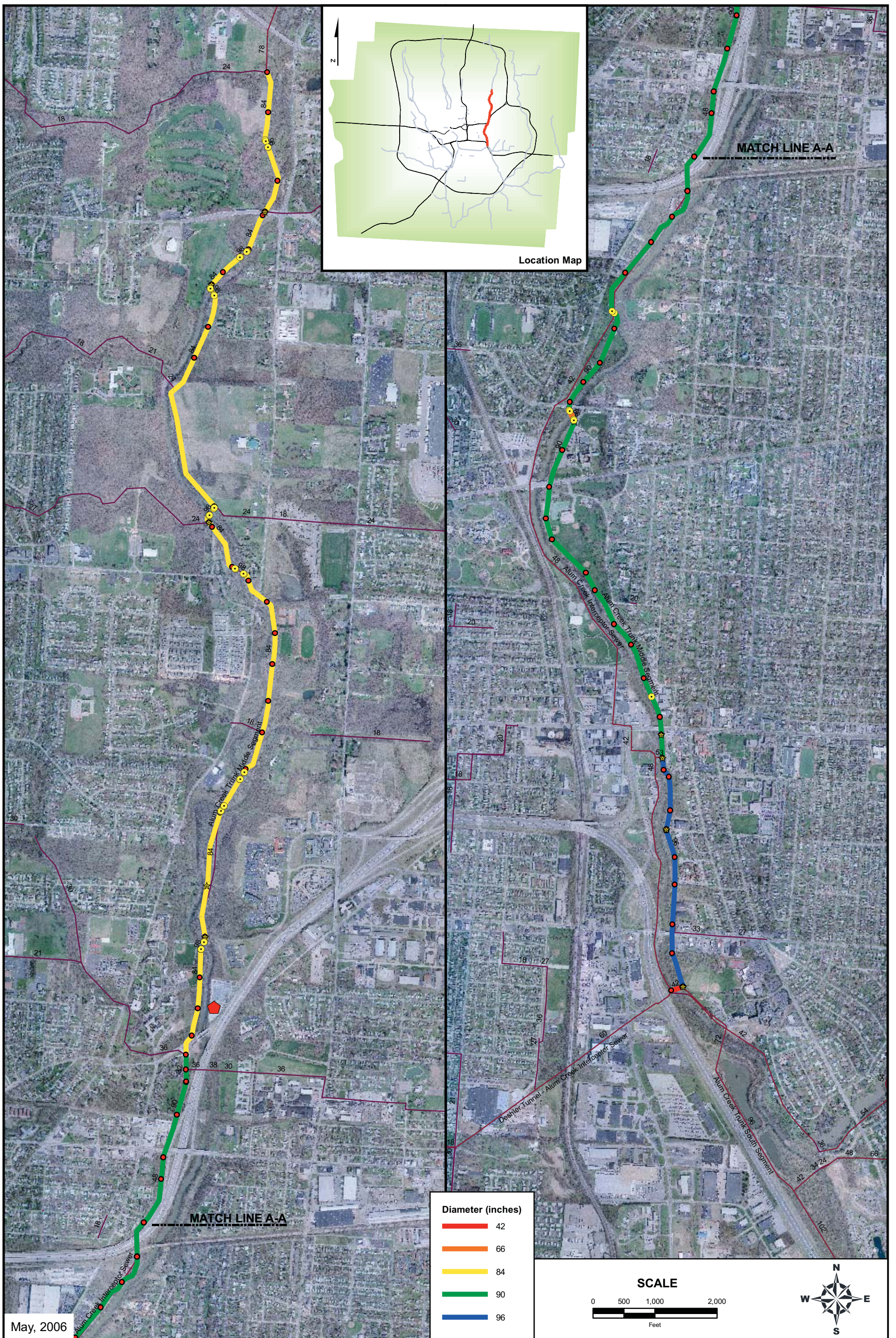
Figure M-3.2 Aerial Plan Alum Creek Trunk Sewer (Middle)
