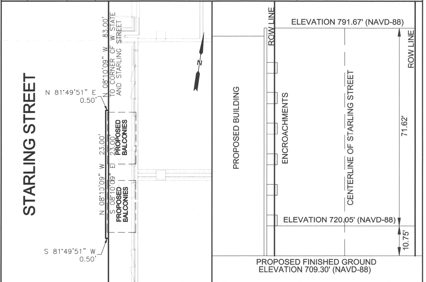
DETAIL - 1"=10'
