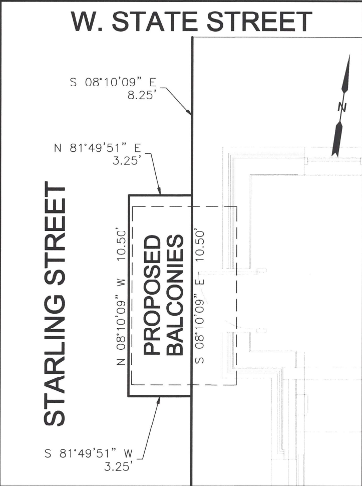
DETAIL - 1"=5'
