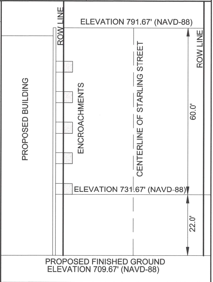
BALCONY LOCATIONS - 1"=20'
