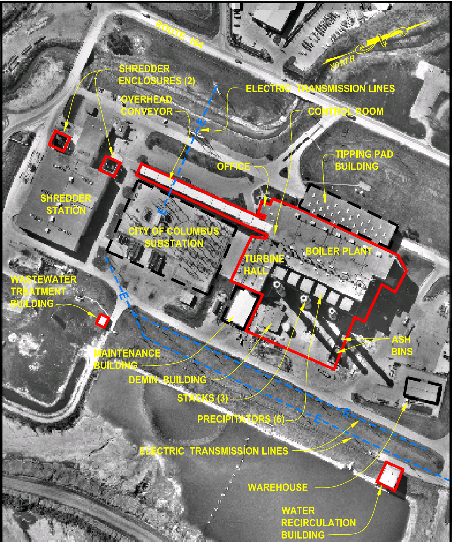
FIGURE 1 GENERAL DEMOLITION PLAN
