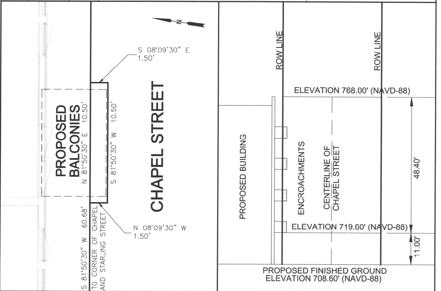
DETAIL - 1"=5'
