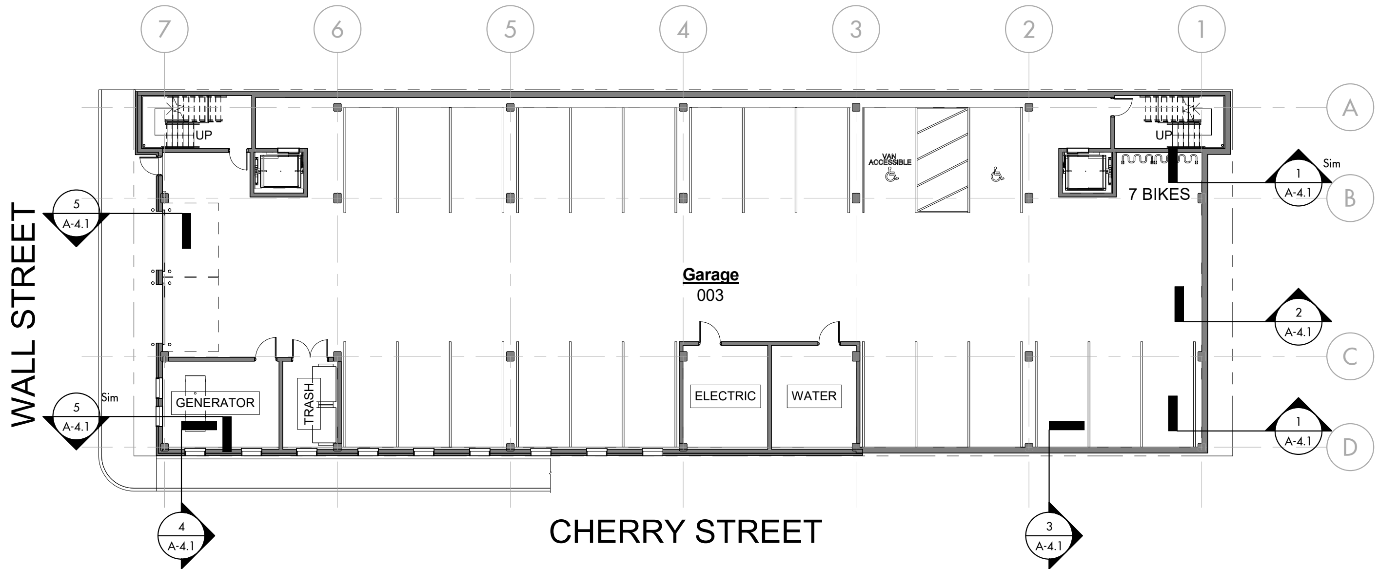
Floor 0 Plan 1/16" = 1'-0"
