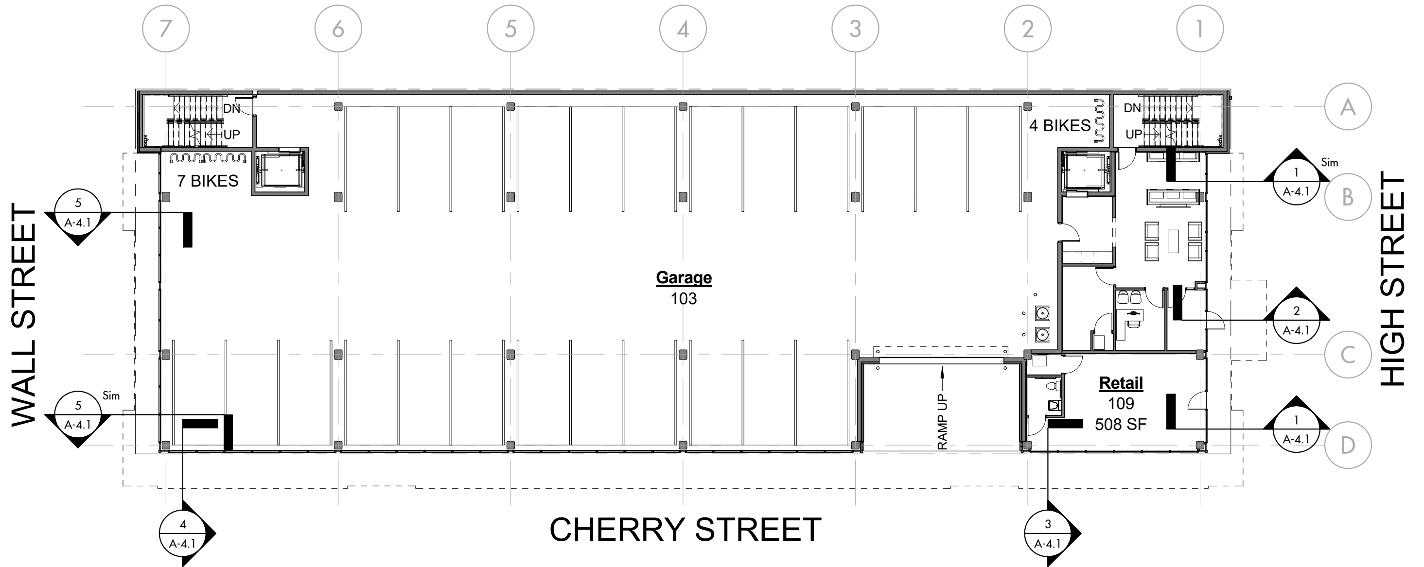
Floor 1 Plan 1/16" = 1'-0"
