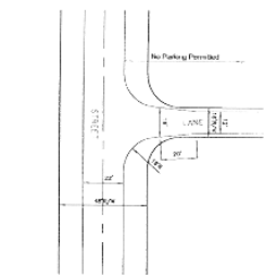
TYPICAL PAVEMENT INTERSECTION FOR STREET/ALLEY
