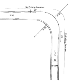
TYPICAL PAVEMENT FOR A 90 DEGREE ALLEY
