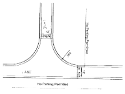
TYPICAL PAVEMENT INTERSECTION FOR ALLEY
