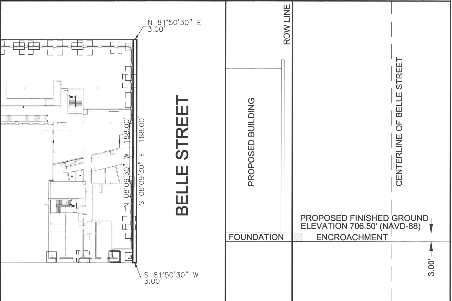
DETAIL - 1"=50'
