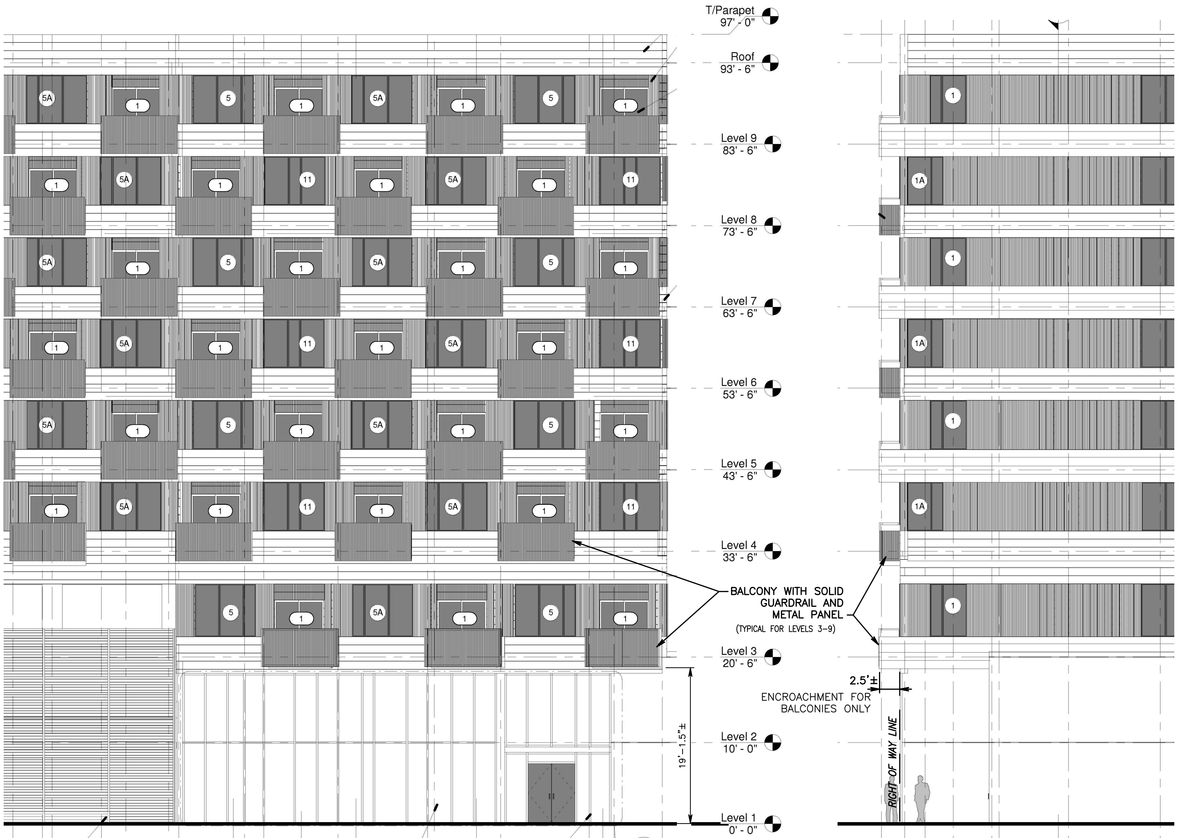
PARTIAL NORTH ELEVATION NOT TO SCALE
