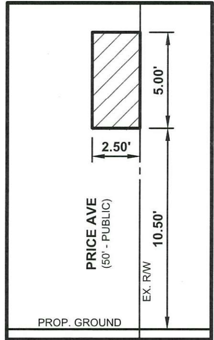
VERTICAL DETAIL (SCALE: 1" = 5')
