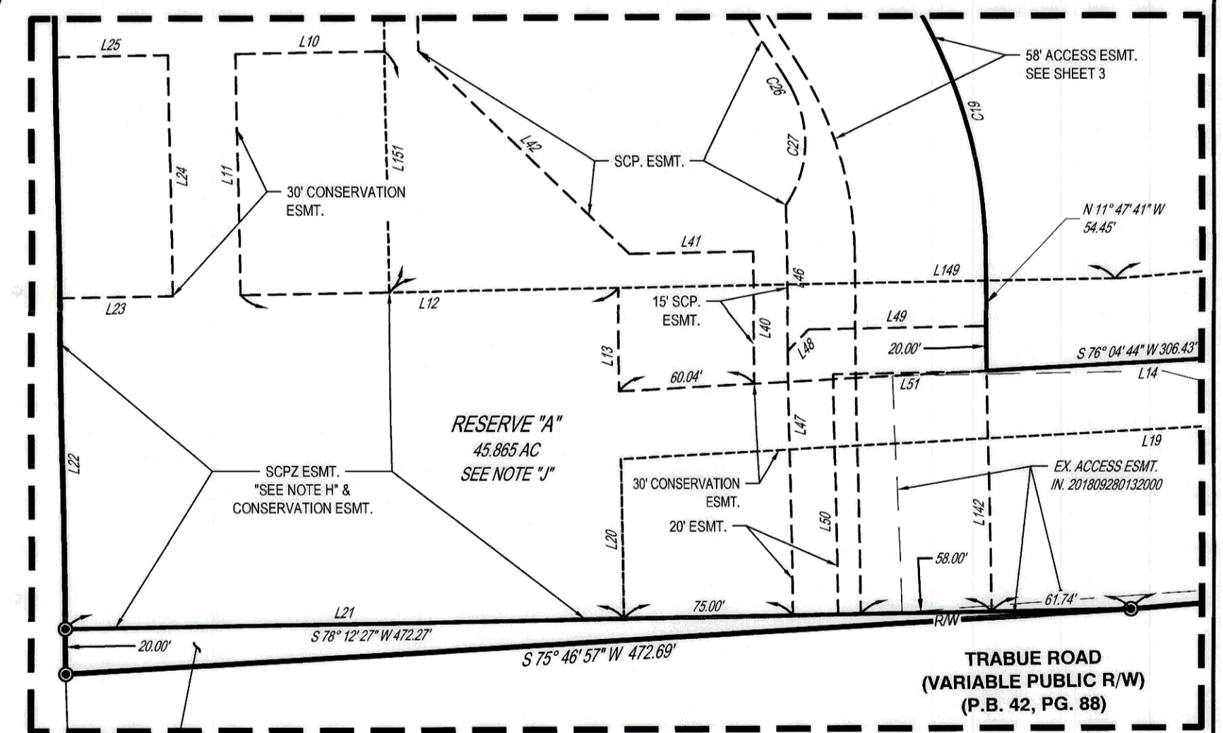
DETAIL "B" SCALE 1" = 60'
